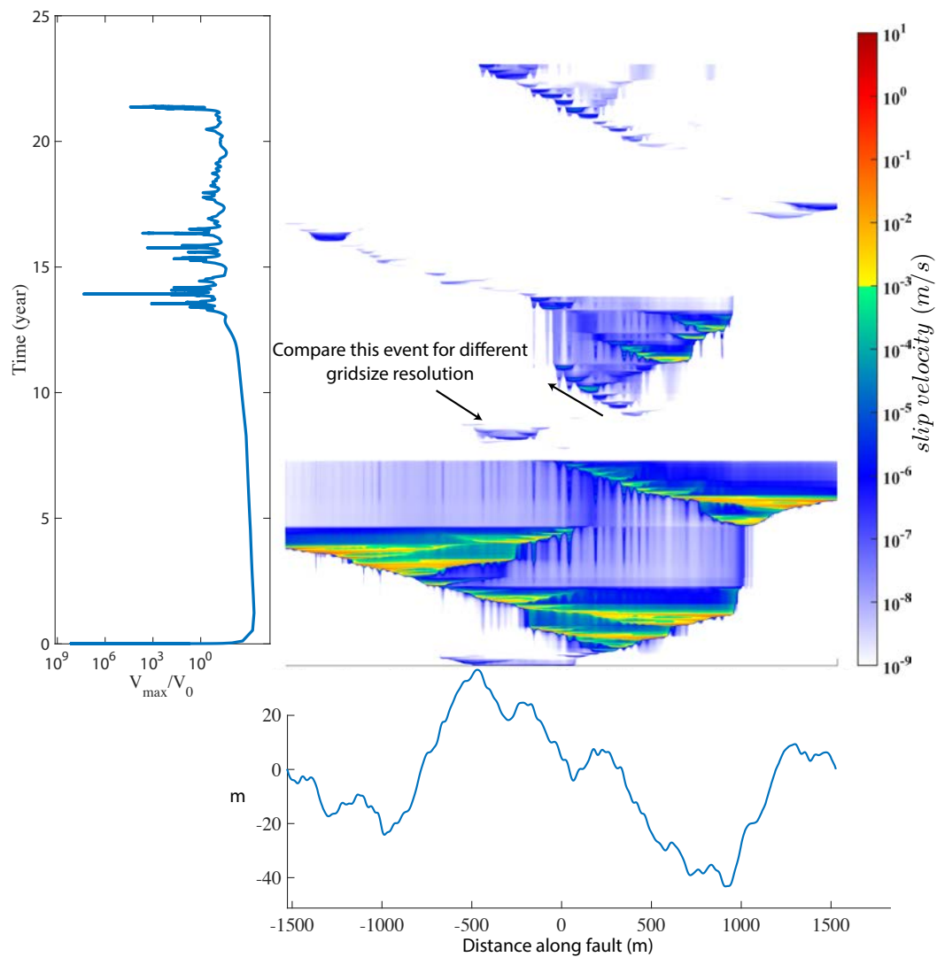
Figure 4.6 – Example of a rough fault in in-plane configuration. Here the amplitude to wavelength ratio is \alpha = 0.01 . Compare to figure 4.5, the number of point used to discretized the fault was doubled.
