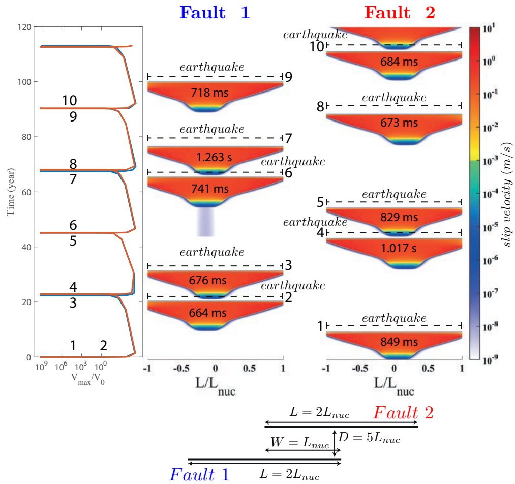
Figure 3.16 – Here the ratio is a/b = 0.8 , the length of the fault is L = 2L_{\text{nuc}} and the distance between the fault D/L_{\text{nuc}} = 5 . Although the fault are quite far, their rupture time is close to each other like if they were synchronizing.
