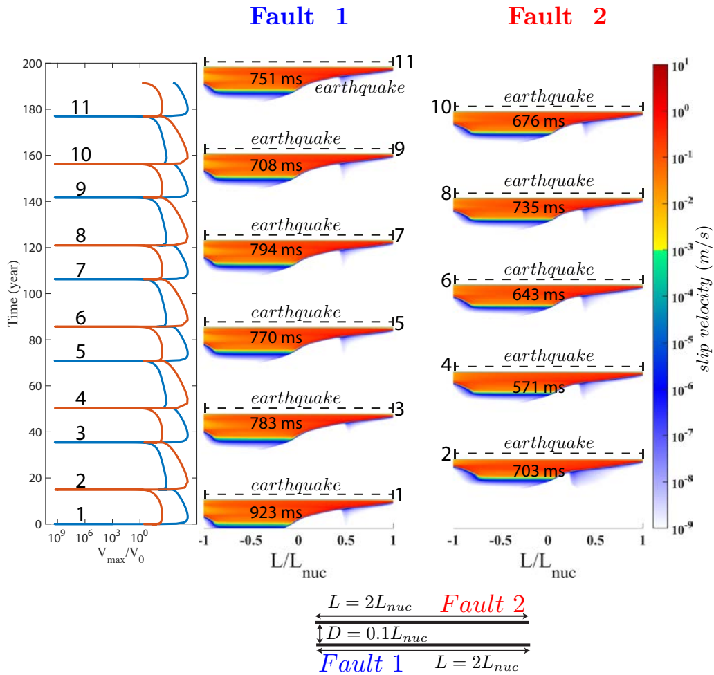
Figure 3.17 – Here the ratio is a/b = 0.8 , the length of the fault is L = 2L_{\text{nuc}} and the distance between the fault D/L_{\text{nuc}} = 0.1 .
