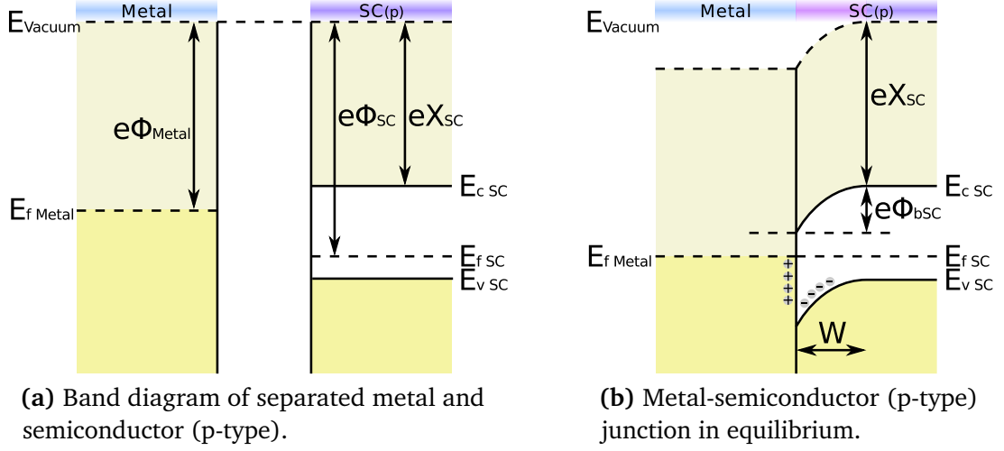
Figure 2.19: Band diagram of metal and semiconductor (p-type) separately and in contact ( \phi_{\text{Metal}} < \phi_{\text{SC}} ). The E_{\text{Vacuum}} is the vacuum level for both systems. E_{f\text{ Metal}} denotes the Fermi level of metal and E_{f\text{ SC}} the Fermi level of the semiconductor. E_{v\text{ SC}} and E_{c\text{ SC}} are the valence band and conduction band edges of the semiconductor, respectively. \phi_{\text{Metal}} and \phi_{\text{SC}} are the work functions of metal and semiconductor, whereas X_{\text{SC}} is the electron affinity of the semiconductor. After creation of a junction the \phi_{bM} and \phi_{bSC} are the barrier heights relative to the metal and semiconductor side, respectively. W denotes the depletion region.
