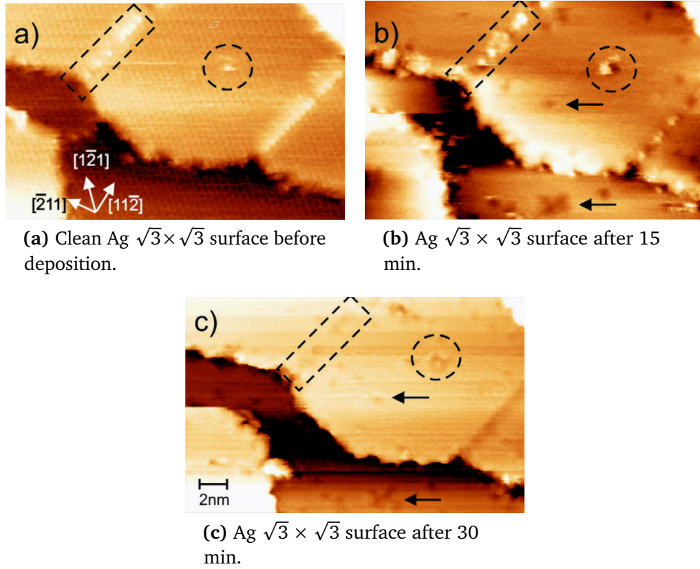
Figure 3.13: The STM images taken during evaporation of FDT at RT at +2 V and 0.25 nA of size 25x16 nm 2 . The preferred adsorption positions, which changed contrast from bright to dark during deposition, were found at defects sites, that is at domain walls (emphasised by rectangle) and point defects (emphasised by circle). Adsorption of FDT on flat terraces (shown with arrows) will be discussed in following parts [TSP10].
