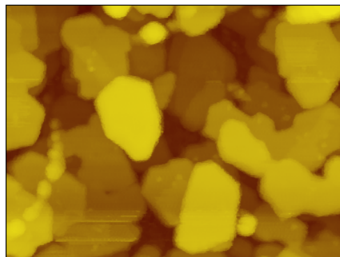
(f) Si(111) Ag \sqrt{3} \times \sqrt{3} with multilayer Ag clusters, annealed.
