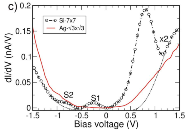
Figure 2.11: Comparison of experimentally obtained LDOS from clean \text{Si}(111) 7 \times 7 surface and \text{Ag } \sqrt{3} \times \sqrt{3} reconstruction [SPT09]. Complete structural and electronic reconstruction is supported by disappearing of the Si characteristic peaks.
