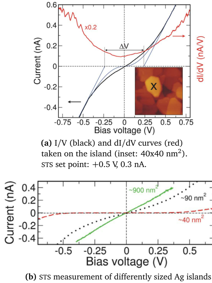
Figure 3.27: STM and STS measurement of the crystalline well ordered Ag islands grown on an Ag wetting layer. The voltage gap \Delta V in (a) is intimately related to the capacitance C of the tunnel junction through \Delta V = e/C . The blue lines represent asymptotes at high biases and a quadratic fit in the low bias regime using R_t = 1 \text{ G}\Omega and C = 0.4 \text{ aF} . (b) [SPT09].
