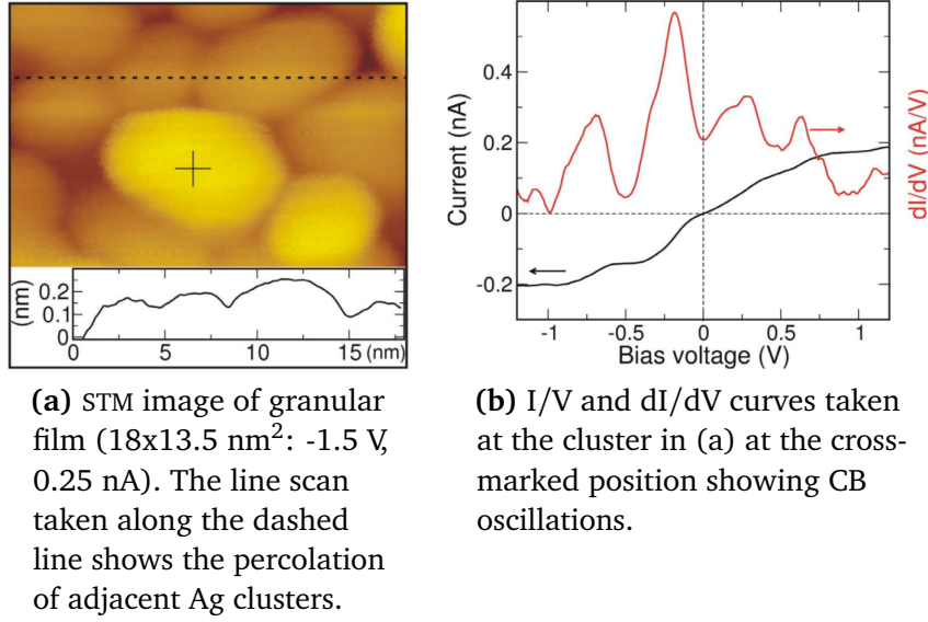
Figure 3.26: 3 ML Ag film annealed to 300 K forming a granular film structure on Si(111) [SPT09].
