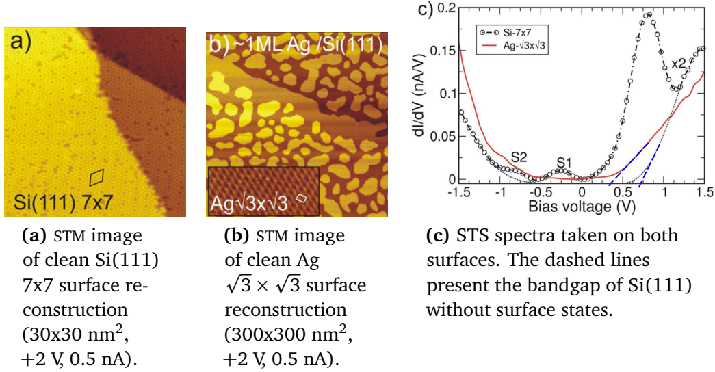
Figure 3.21: STM images of clean Si(111) and Ag \sqrt{3} \times \sqrt{3} surfaces and respective STS measurement of both surfaces. Inset in (b): Ag islands (size 7.4 \times 3.2 \text{ nm}^2 , +1 V, 0.4 nA) [SPT09].
