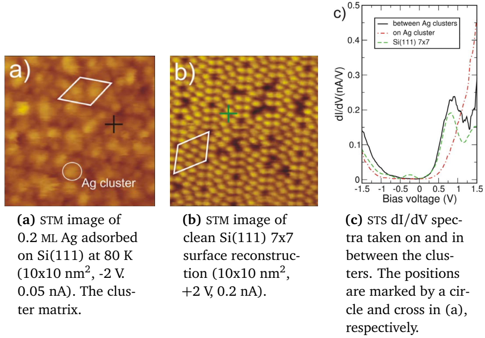
Figure 3.23: The comparison with the corner hole structure of the clean Si(111) surface (b) shows that the Ag clusters on (a) are aligned along the 7x7 reconstruction. The unoccupied Si-surface state is visible in between the Ag clusters. For comparison, the spectrum of the clean surface is shown as dashed green line [SPT09].
