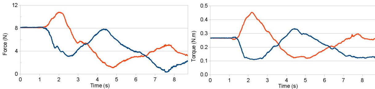
Fig. 11. Bimanual coupling on the same rigid body. Plot of the force (left) and the torque (right) generated by fluid inside a bucket coupled to two 6DoF haptic devices (left hand in red/light, right hand in blue/dark). The peaks and valleys correspond to the tilting movements, increasing the force and the torque on the side to which the bucket is tilted. Forces and torques progressively decrease as fluid is spilled.
